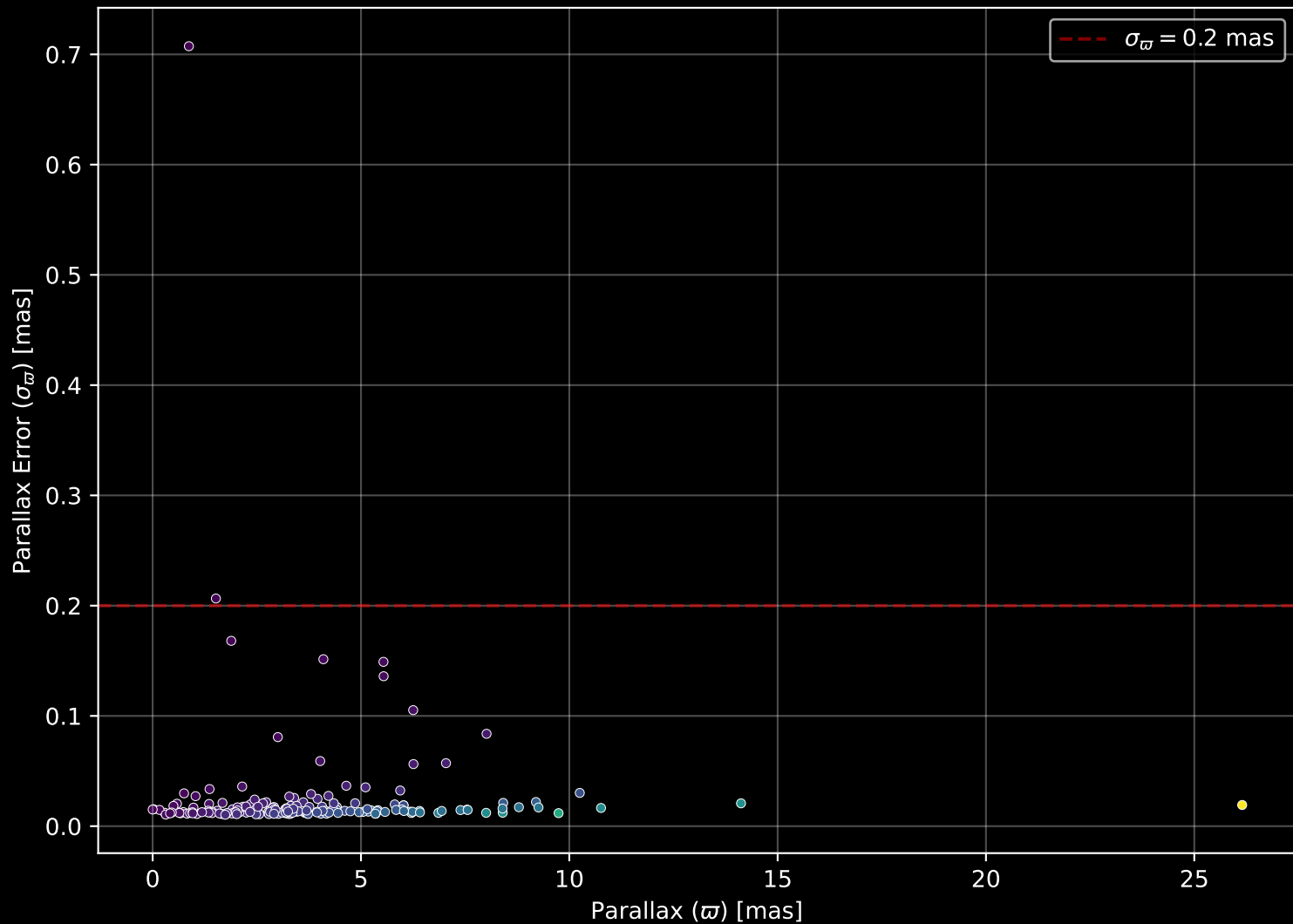
APOGEE DR17 Field: [055+63_MGA] Parallax Quality (n= 177)
