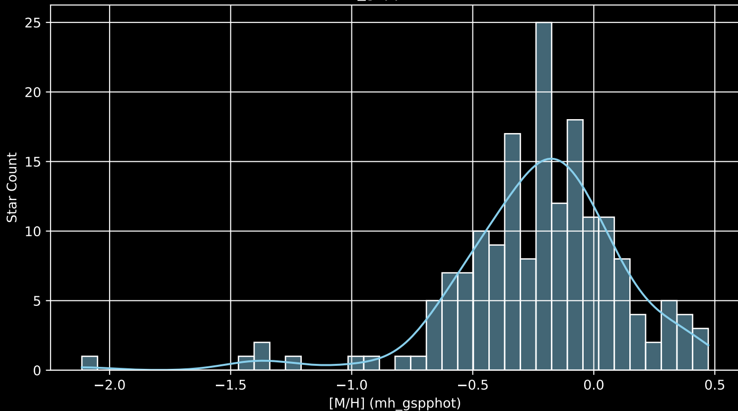
APOGEE DR17 Field: [055+63_MGA [M/H] (mh_gspphot) (n= 175)
