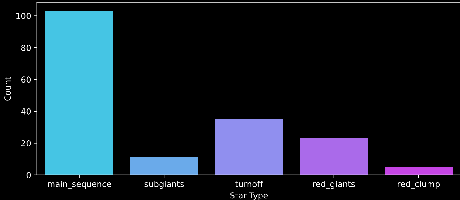
APOGEE DR17 Field: [055+63_MGA] Count plot of Star Type
