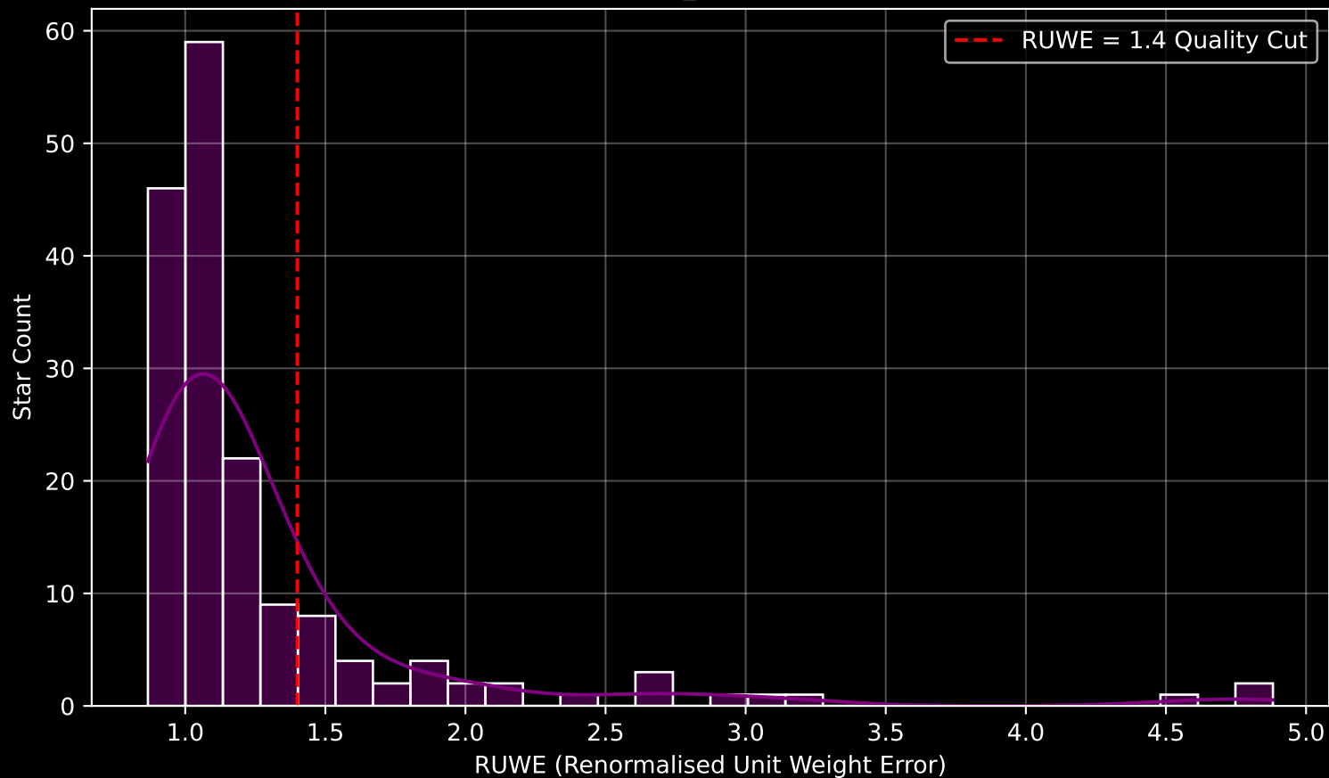
GAPOGEE DR17 Field [055+63_MGA] RUWE Distribution (n= 168)
