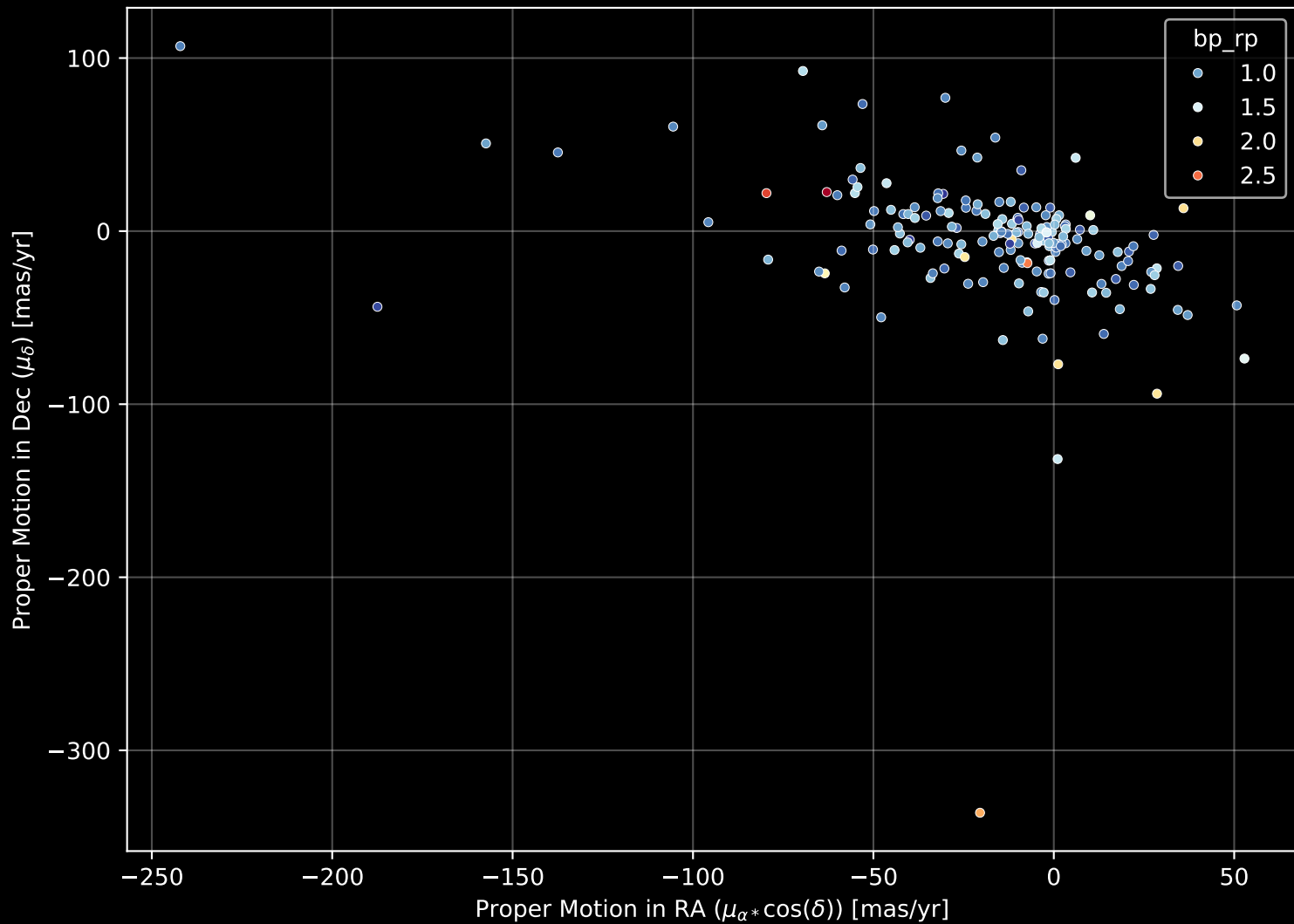
APOGEE DR17 Field: [055+63_MGA] Proper Motion Diagram (n= 177)
