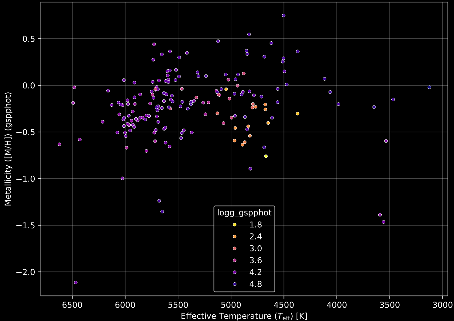
APOGEE DR17 Field: [055+63_MGA] Stellar Population Parameters (n= 177)
