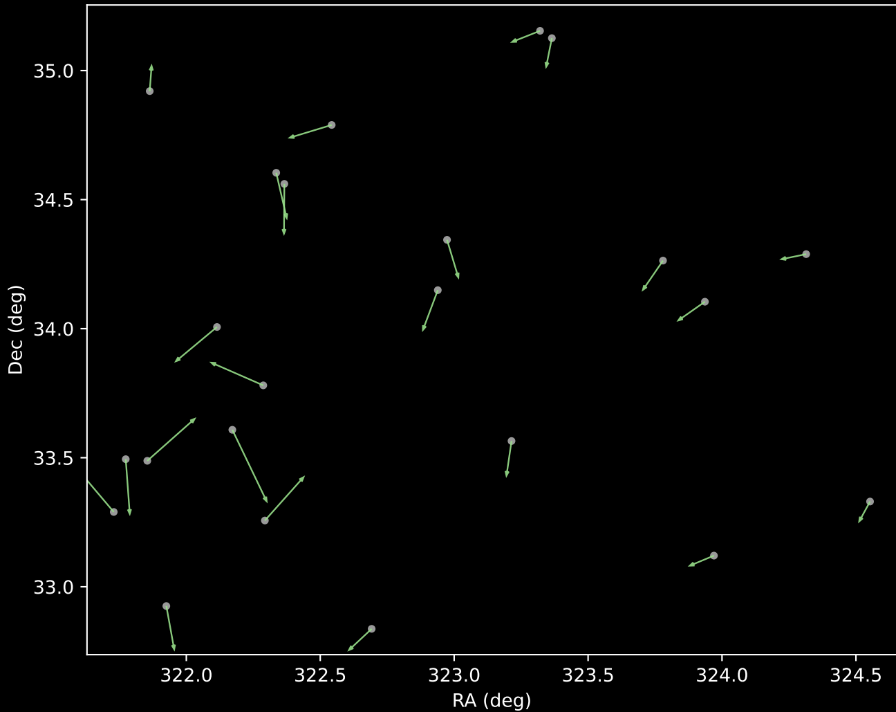
APOGEE DR17 Cluster 5 Proper Motion Vectors (n=23)
